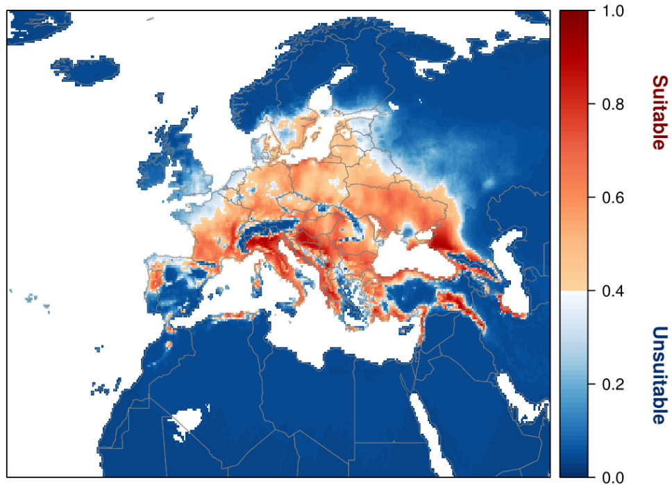
Figure 5. Projected current suitability for Lespedeza cuneata establishment in Europe and the Mediterranean region. The white areas have climatic conditions outside the range of the training data so were excluded from the projection.
