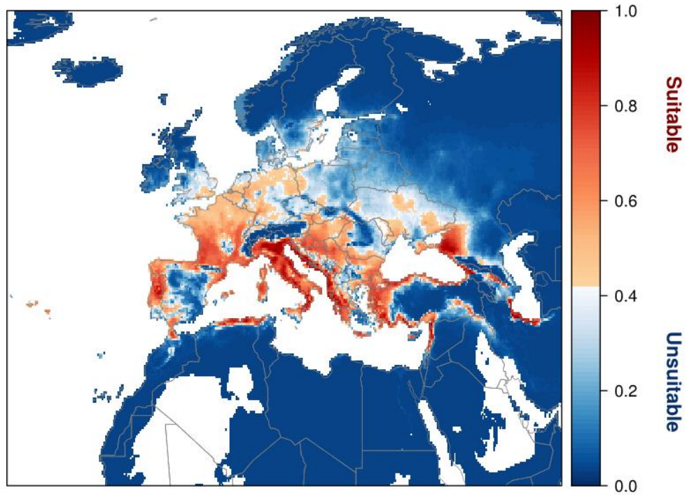
Figure 7. Projected suitability for Triadica sebifera establishment in Europe and the Mediterranean region in the 2070s under climate change scenario RCP4.5, equivalent to Figure 5.
